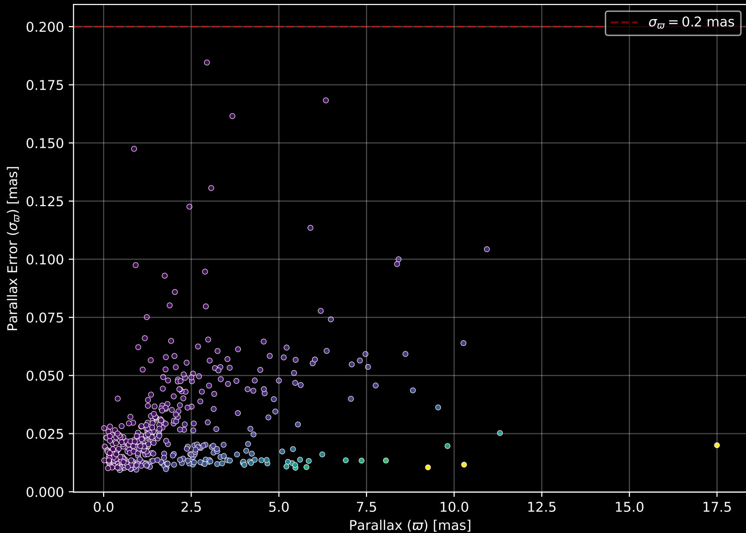
APOGEE DR17 Field: [120+45] Parallax Quality (n= 420)
