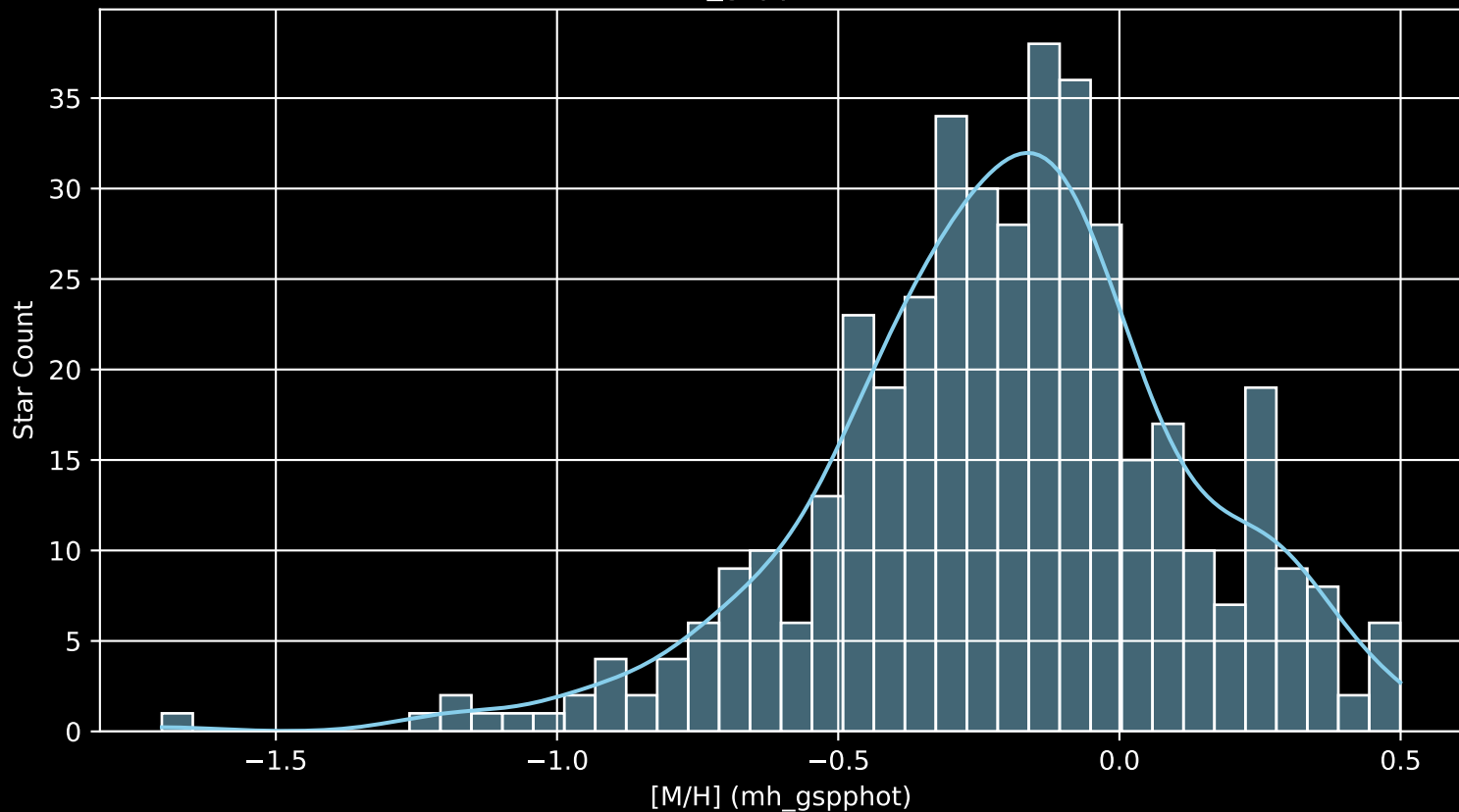
APOGEE DR17 Field: [120+45 [M/H] (mh_gspphot) (n= 416)
