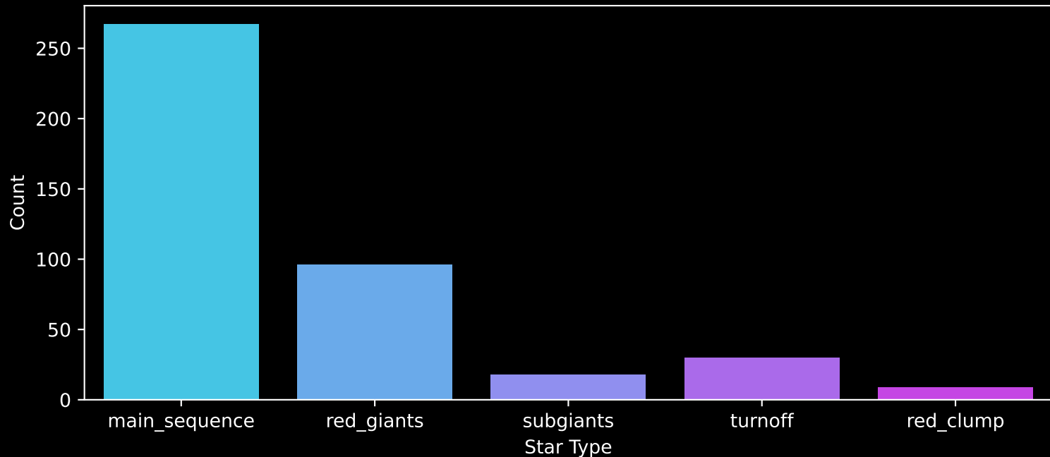
APOGEE DR17 Field: [120+45] Count plot of Star Type
