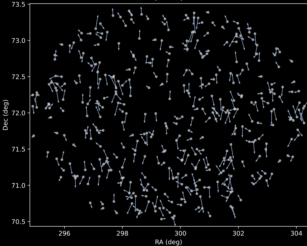
APOGEE DR17 Cluster 1 Proper Motion Vectors (n=376)
