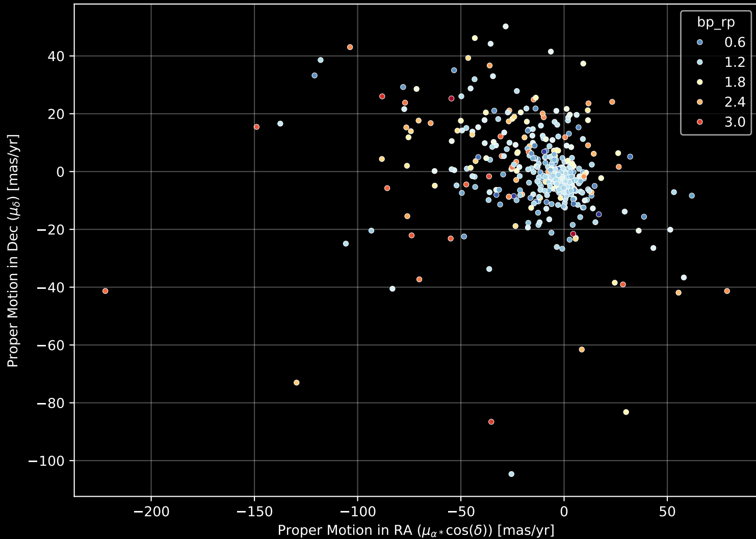
APOGEE DR17 Field: [120+45] Proper Motion Diagram (n= 420)
