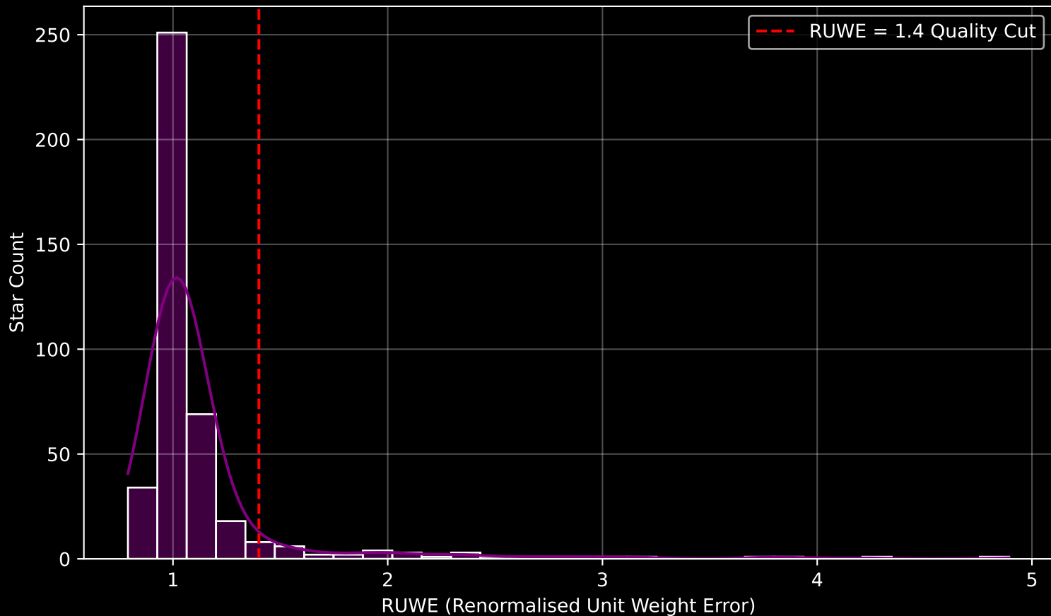
GAPOGEE DR17 Field [120+45] RUWE Distribution (n= 411)
